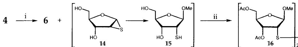
Scheme 1 Reagents and conditions: i, NaOMe, MeOH, reflux, 2 hr; ii, Ac 2 O, C 6 H 5 N, RT
